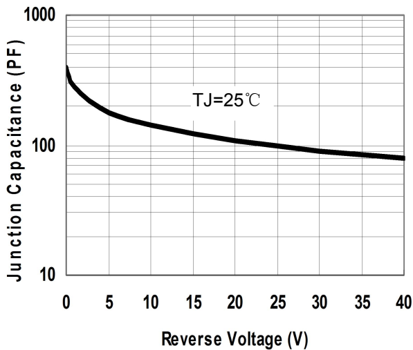
Fig.1-Typical Junction Capacitance
